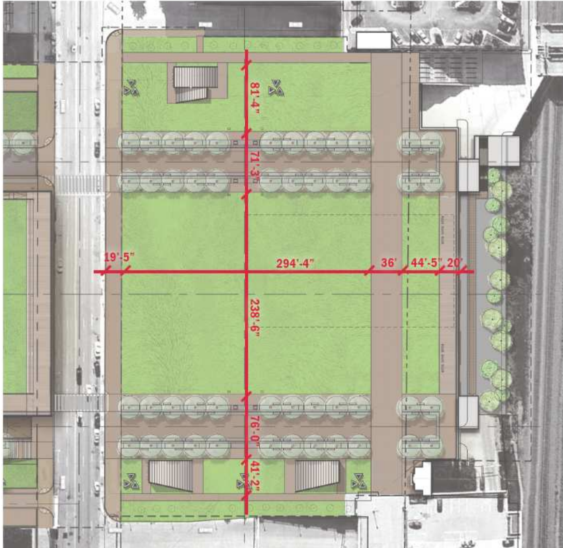
SITE PLAN: MALL C
