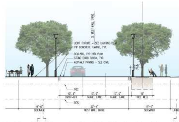
2 - Section through West Mall Drive (Curbless at Drop-off)
