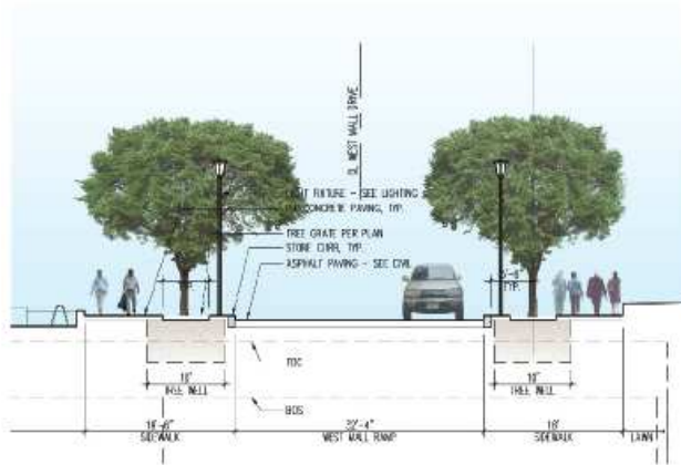
1 - Section through West Mall Drive (Curbs)
