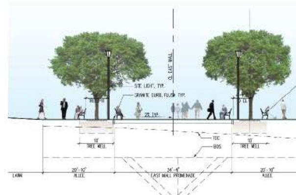
3 - Section through East Mall Promenade
